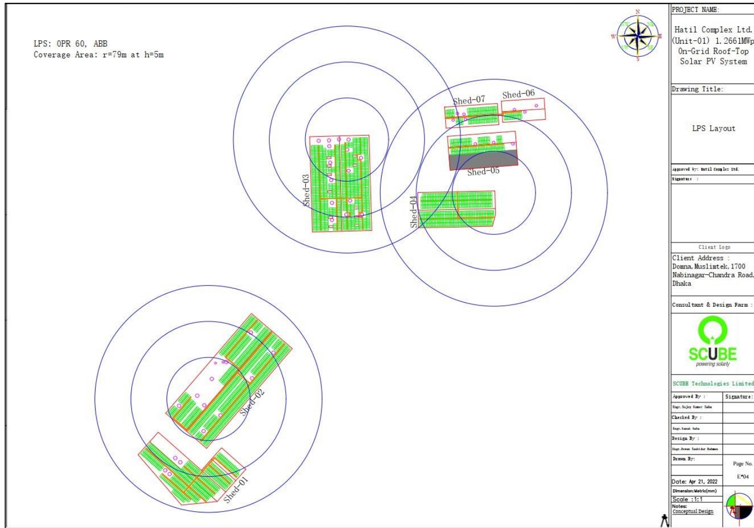
Figure 12: Lighting Protection System of Rooftop Solar PV (Unit-01)
