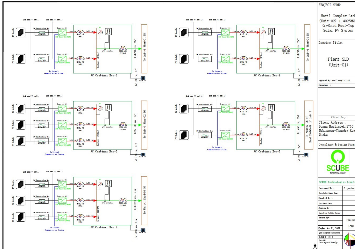
Figure 10: Plant Single Line Diagram of Unit-01
