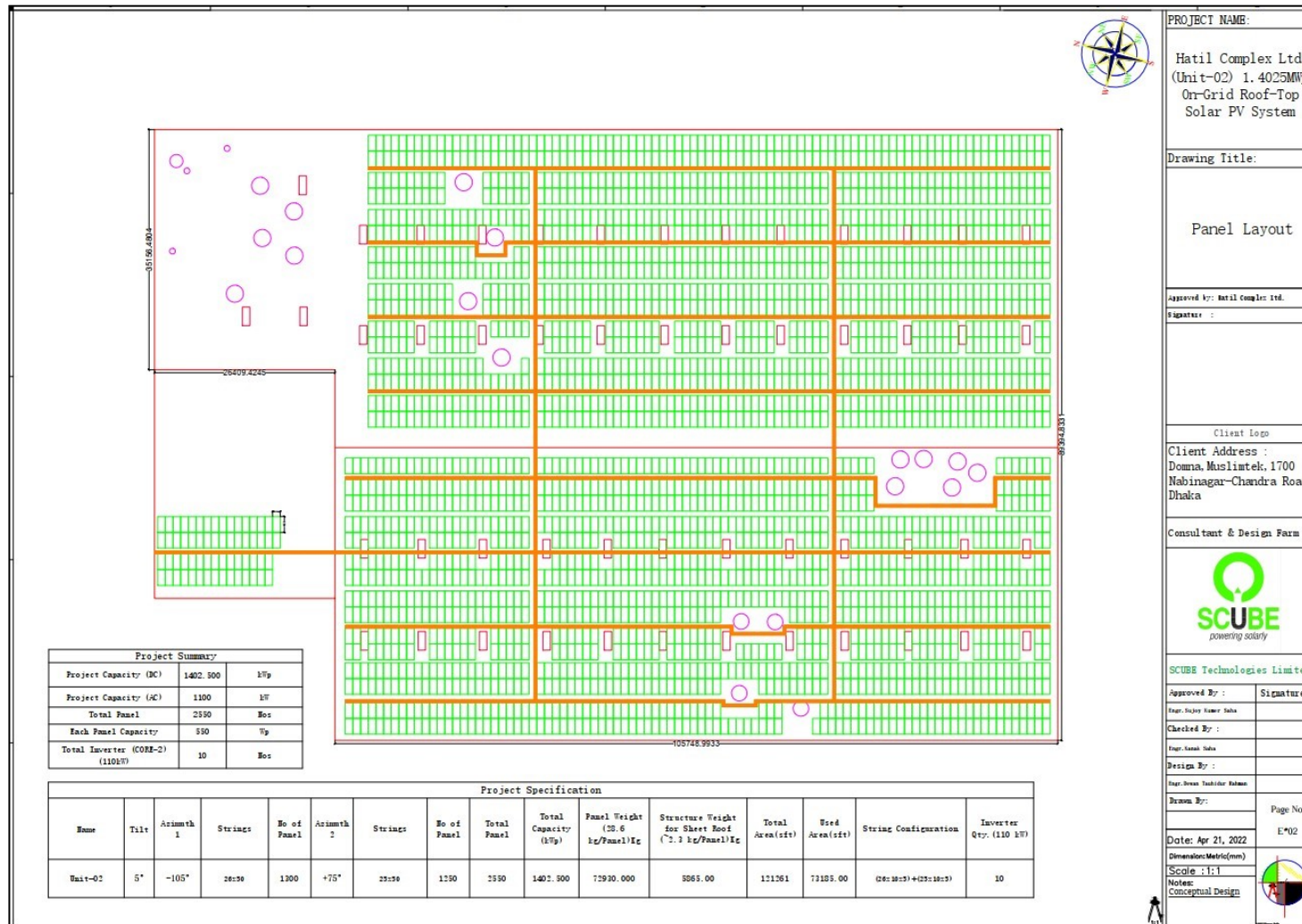
Figure 9: Panel Layout Plan of Unit-02
