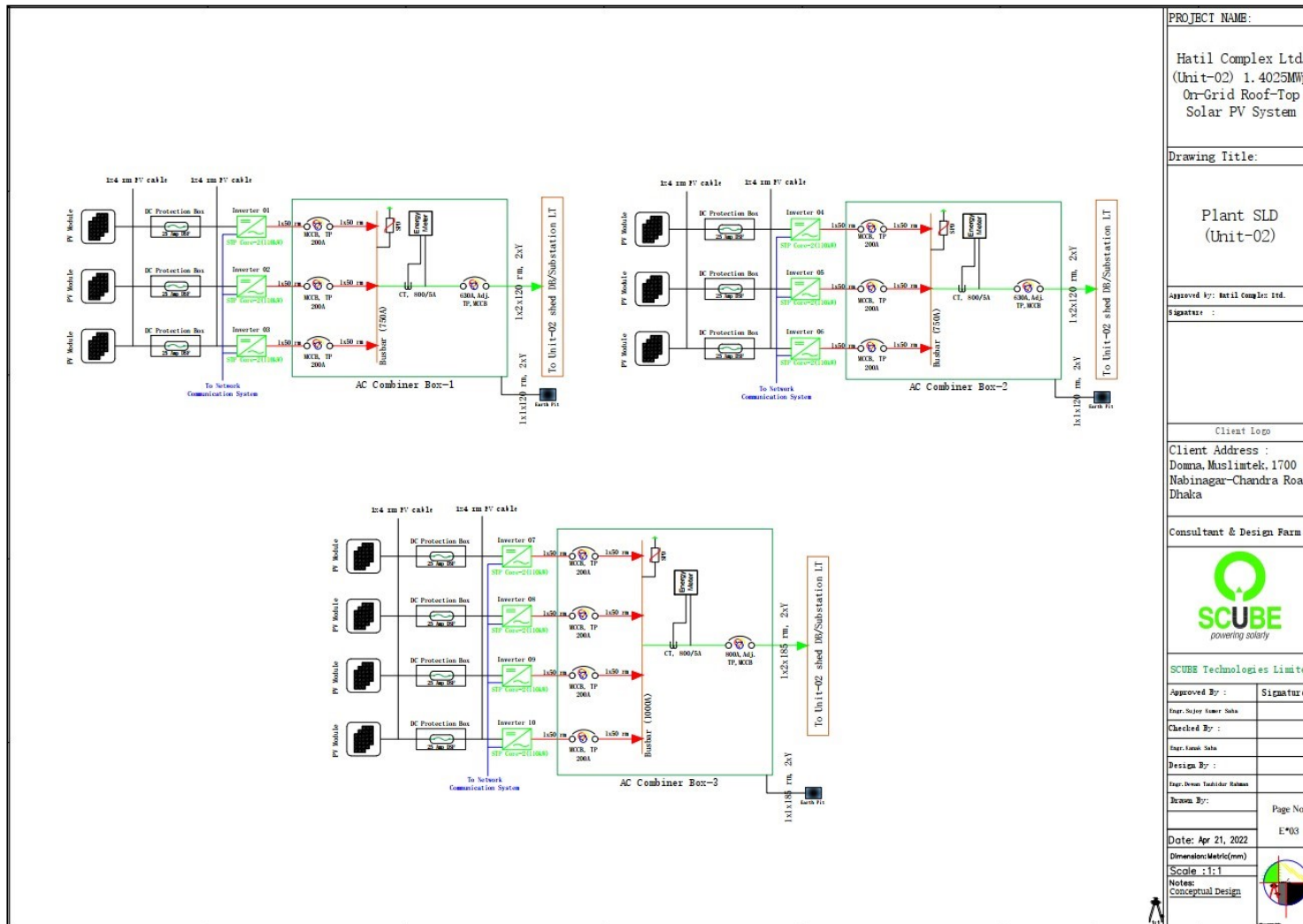
Figure 11: Plant Single Diagram of Unit-02
