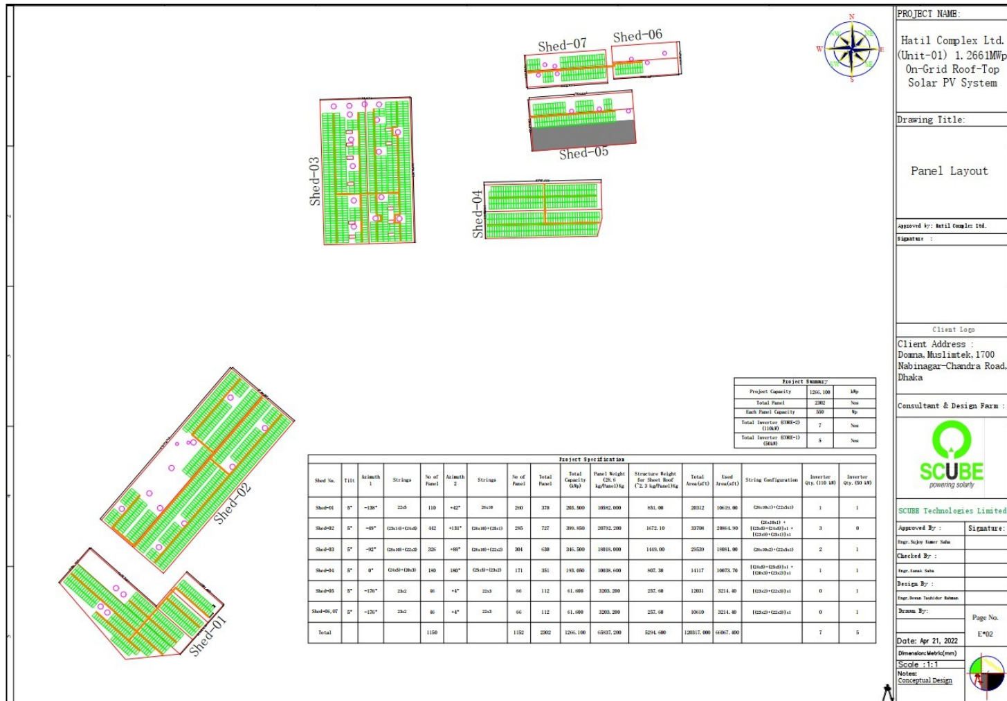
Figure 8: Panel Layout Plan of Unit-01
